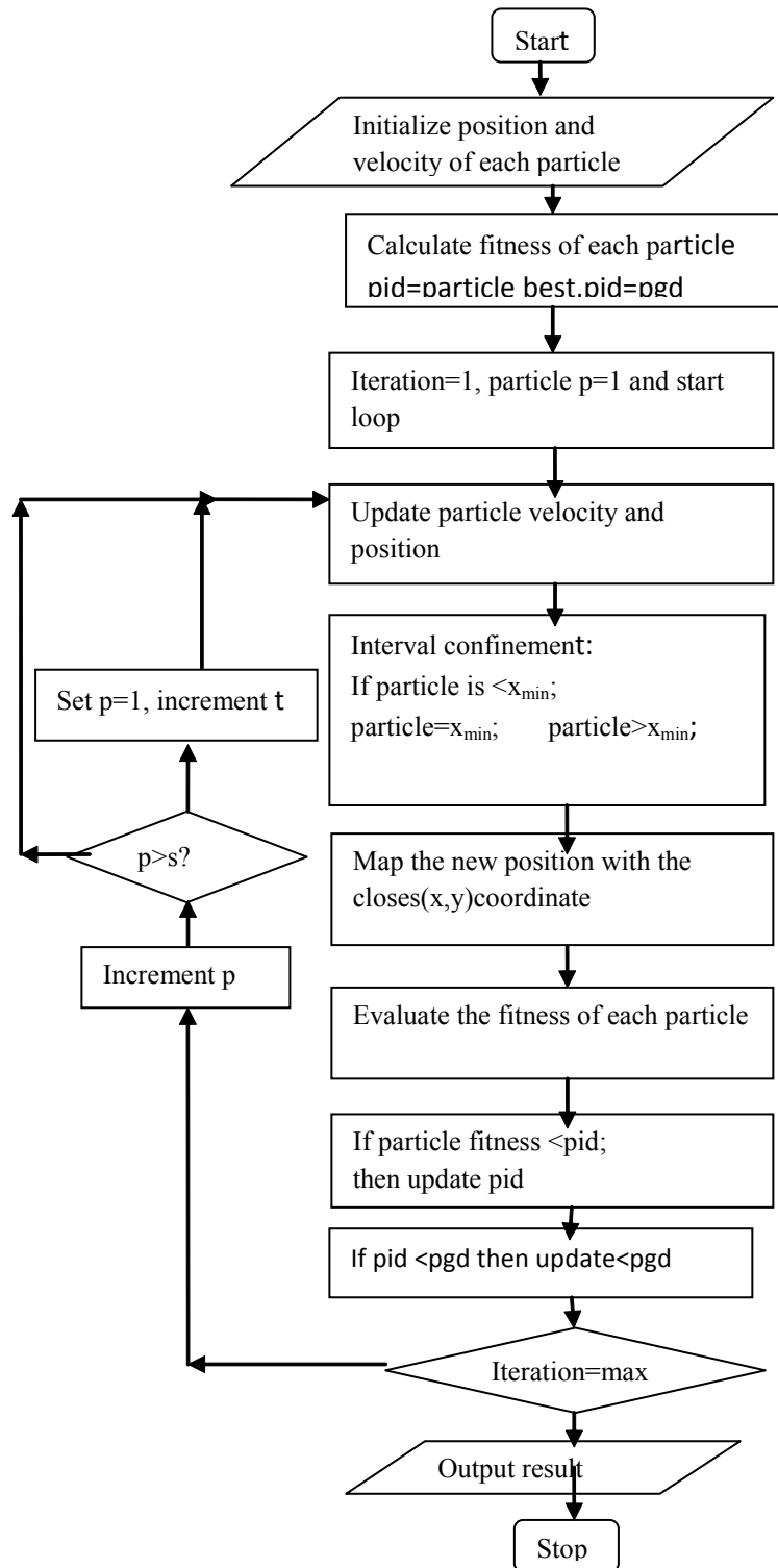
Fig. 1: Flowchart of PSO
